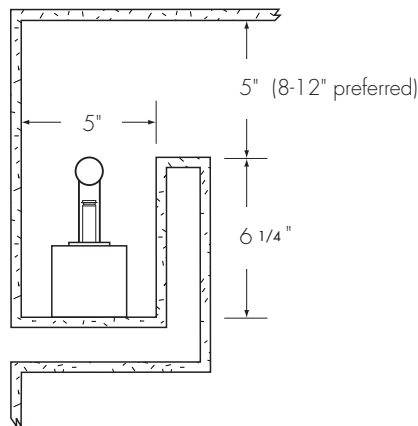
BL (surface-mounted) lampholder mounted to a horizontal surface
