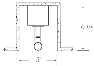
BL (surface-mounted) lampholder mounted in a downward-hanging configuration
