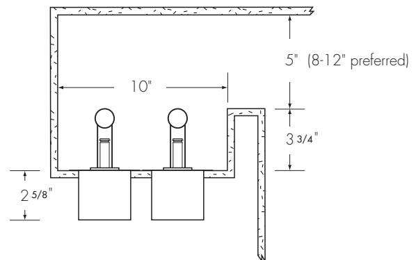
A double row of BL-R (recess-mounted) lampholders mounted to a horizontal surface
