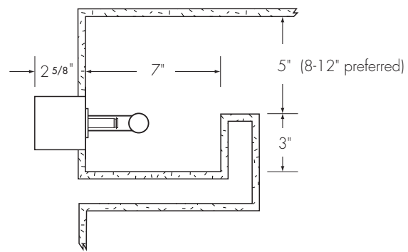
BL-R (recess-mounted) lampholder mounted to a vertical surface
