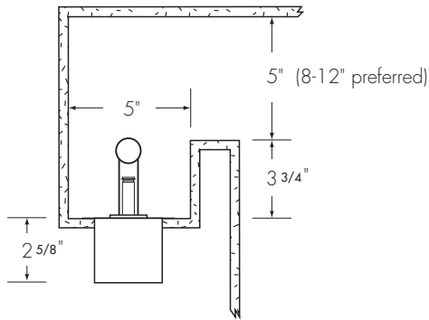
BL-R (recess-mounted) lampholder mounted to a horizontal surface
