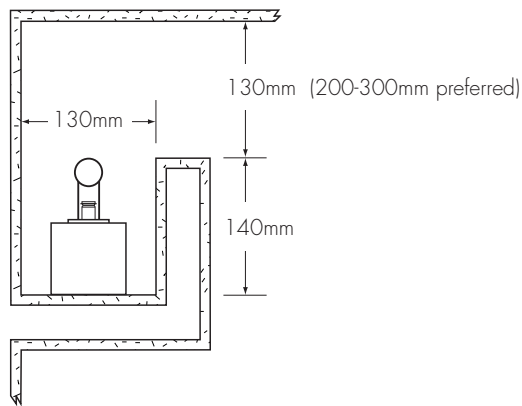
BL (surface-mounted) lampholder mounted to a horizontal surface
