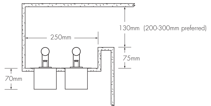
A double row of BL-R (recess-mounted) lampholders mounted to a horizontal surface
