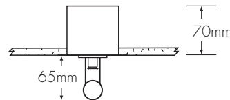
BL-R (recess-mounted) lampholder mounted to a horizontal surface for an exposed sculptural lamp application
