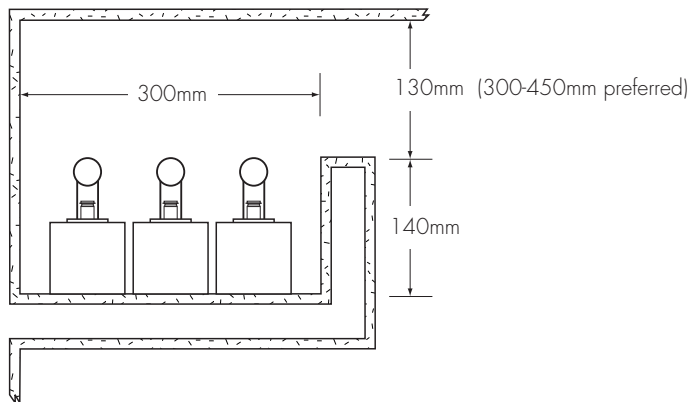
A triple row of BL (surface-mounted) lampholders mounted to a horizontal surface
