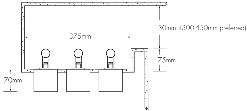
A triple row of BL-R (recess-mounted) lampholders mounted to a horizontal surface
