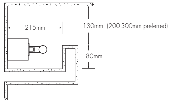
BL (surface-mounted) lampholder mounted to a vertical surface
