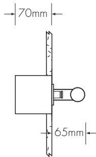
BL-R (recess-mounted) lampholder mounted to a vertical surface for an exposed sculptural lamp application
