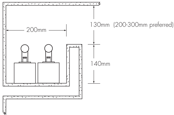
A double row of BL (surface-mounted) lampholders mounted to a horizontal surface
